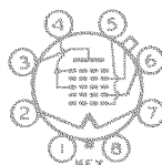
BOTTOM VIEW (G-7Z)
